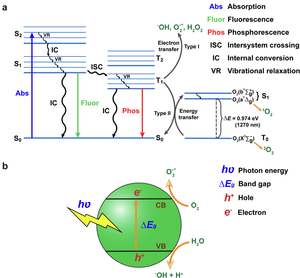
Fig. 2. Underlying principles of PDT and PTT. (a) The Jablonski diagram demonstrates the general mechanism of reactive oxygen species and free radical generation in PDT and PTT upon photon absorption (abs) by a photosensitizer or photothermal agent, respectively. Following photon absorption, electrons are promoted from the ground state ( S_0 ) to an excited singlet state ( S_n ; n \neq 0 ) then relax by emitting energy as heat (VR, IC) or light (fluorescence or phosphorescence). Type I reactions result in the generation of free radicals ( O_2^{\cdot-} , \cdot OH ) and H_2O_2 . Type II reactions result in singlet oxygen generation ( ^1O_2 ). (b) Schematic of free radical generation in metal oxide nanomaterials. Valence electrons are excited from the valence band (VB) to the conduction band (CB) when exposed to light that exceeds the energy of the bandgap. The resulting charge separated state is conducive to energy transfer (type II) reactions producing free radical species, which degrade microbial and viral macromolecules.
