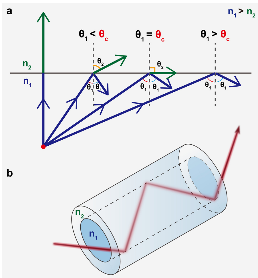
Fig. 4. Schematic illustration of the (a) dependence on incident light angle and refractive index to achieve total internal reflection and (b) light propagation through a step-index optical fiber via total internal reflection resulting in minimal energy loss over the length of the fiber. \theta_1 : incident angle; \theta_2 : transmitted angle; \theta_c : critical angle; n_1 and n_2 : refractive indexes of media 1 and 2, respectively.
